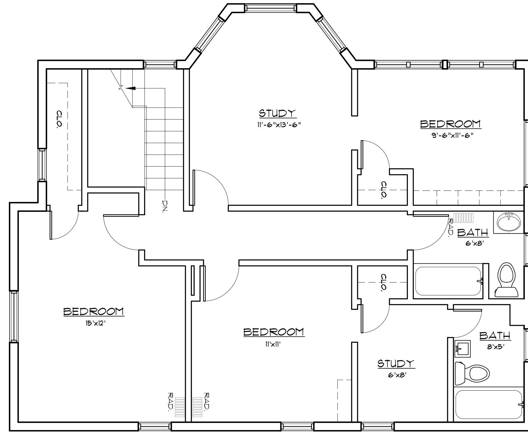
2ND FLOOR SCALE: 1/4" = 1'-0"
