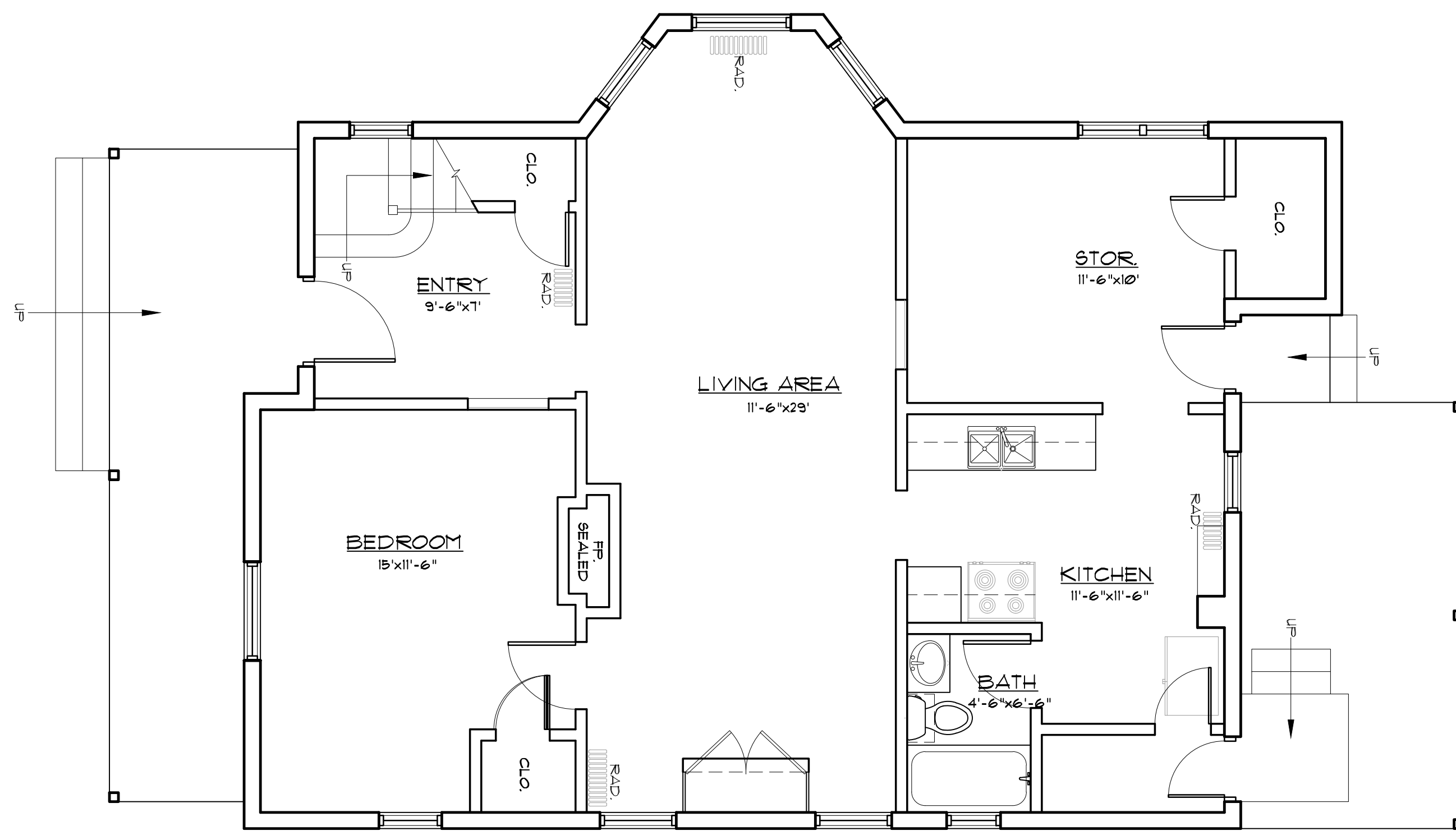
1ST FLOOR SCALE: 1/4" = 1'-0"
