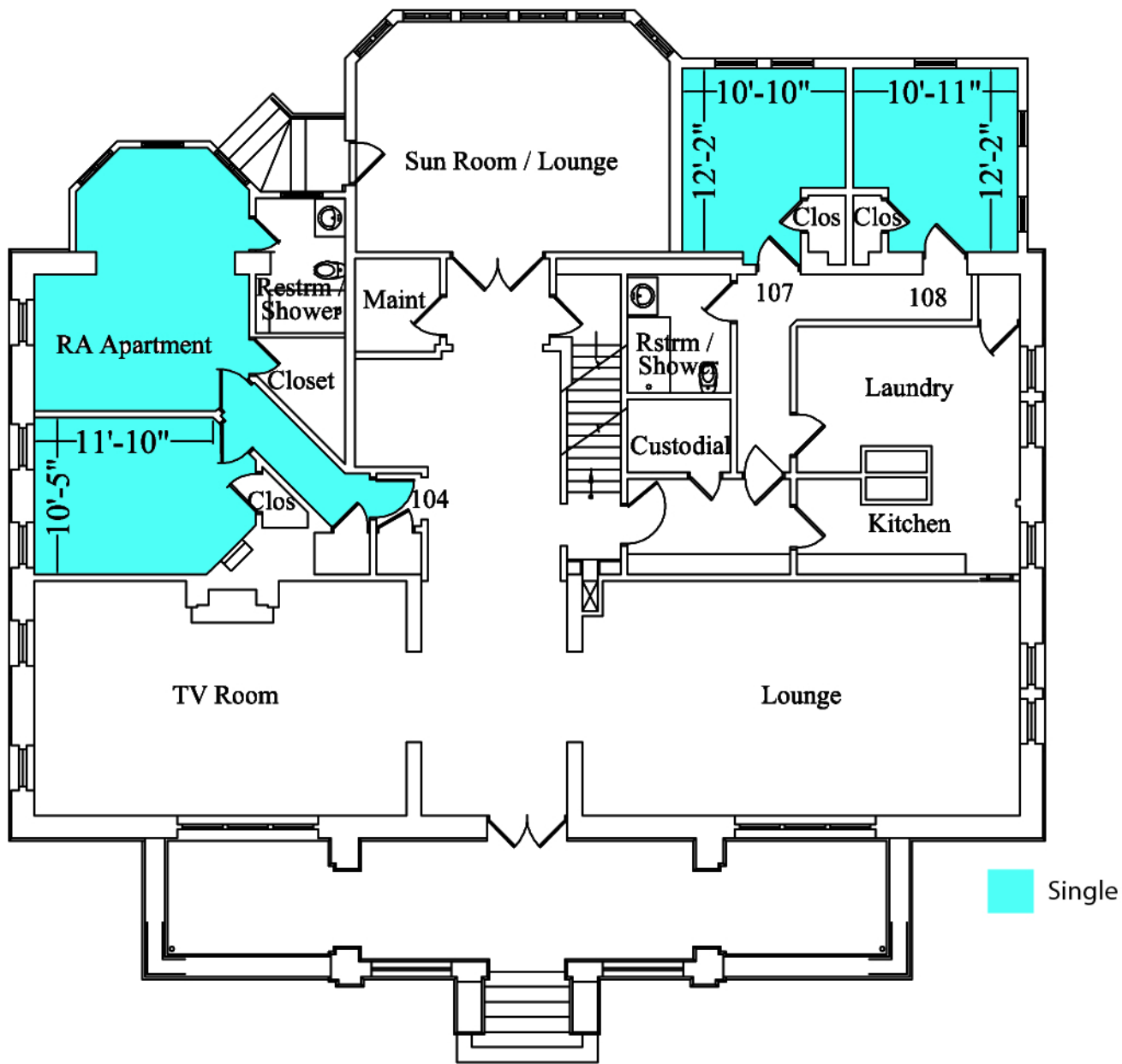
Montgomery House - First Floor Plan
