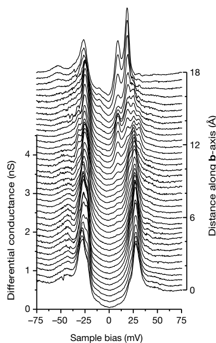
Figure 4 Evolution of the dI/dV spectra and superconducting energy gap as a function of distance from the Ni atom. A series of differential conductance spectra (shifted vertically from each other for clarity), taken as a function of distance away from the centre of a Ni impurity state along the b -axis. The top spectrum is taken above the Ni site. The spectra, each separated by 0.5 Å, show that over a \sim 20 Å range the magnitude of the superconducting gap \Delta_0 = 28 meV, as measured by the separation between the hole-like coherence peak and the Fermi level, is not suppressed in the presence of the Ni impurity. Line cuts approaching the Ni site from other directions lead to the same conclusion. There are variations in \Delta_0 throughout the crystal but this study was carried out in a patch with constant \Delta_0 of 28 meV. The junction resistance was 1 GΩ at -100 mV for all spectra.
