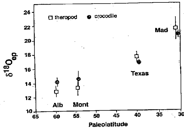
Figure 2. Average \delta^{18}\text{O} of enamel phosphate ( \delta^{18}\text{O}_{\text{ep}} ) \pm 1\sigma for crocodile and theropod teeth versus absolute paleolatitude for localities where both taxa are present. Alb—Albion, Alberta, Mont—Montana, Mad—Madagascar.
